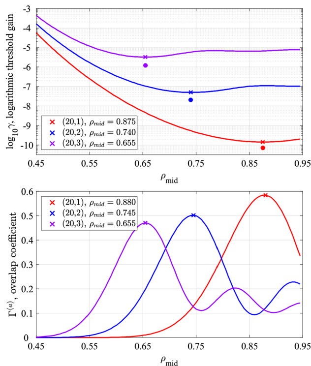
Fig. 4 Dependences of the threshold material gains ( top panel ) and the overlap coefficients ( bottom panel ) on \rho_{mid} for WGMs (20,1), (20,2) and (20,3) of the circular microcavity with the ring-like active region of the width d = 0.1r_3 . The maxima of the overlap coefficients and the minima of the threshold gain are marked with crosses. The threshold gains of the same modes for the fully active circular cavity are indicated with the dots in the top panel
