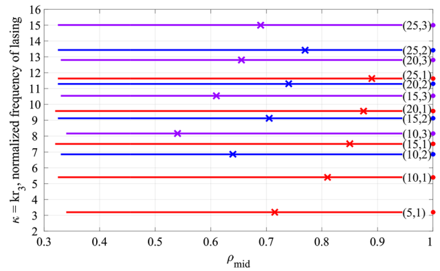
Fig. 3 Same as in Fig. 2 for the lasing frequencies. The values of \rho_{mid} corresponding to the minima of the threshold gains are marked with crosses. The normalized frequencies of lasing of the same modes of the fully active circular microcavity are marked with circles
