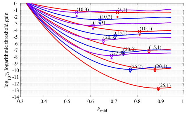
Fig. 2 Dependences of the threshold material gains for the circular microcavity with a ring-like active region on the middle radius of the ring \rho_{mid} . The minimum values of threshold gains are marked with crosses. The threshold gains of the corresponding modes for the fully active circular microcavity are marked with dots
